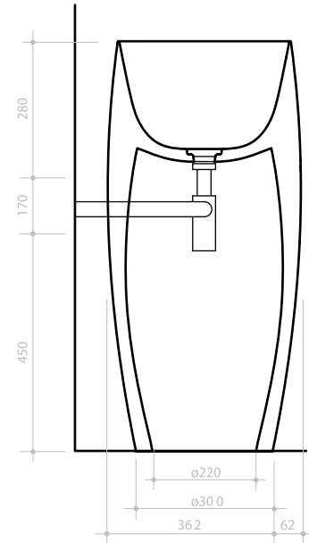
Afvoer langs de wand Evacuation murale Wall/Floor Drainage
